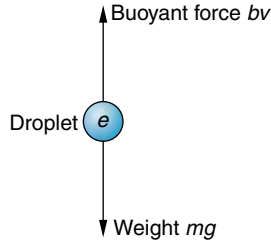
Fig. 3-5 An oil droplet carrying an ion of charge e falling at terminal speed, i.e., mg = bv .
