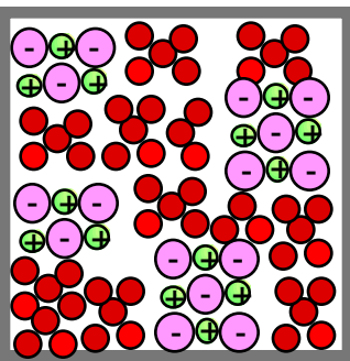
two solids
