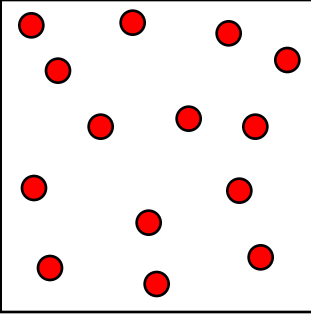
gas
