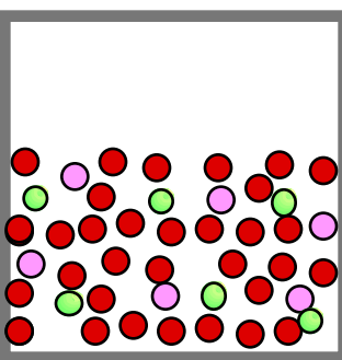
liquid solution
