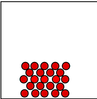
solid
