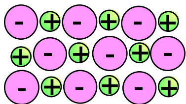
ionic compound
