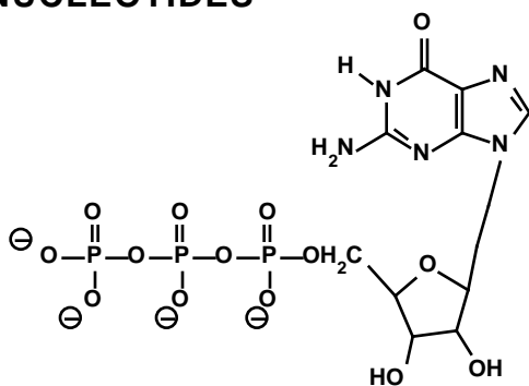
Guanosine-5'-triphosphate (GTP)
