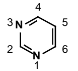
Pyrimidine
