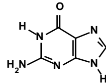
Guanine
