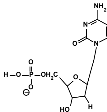
Deoxycytidine-5'-monophosphate (dCMP)
