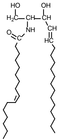
CERAMIDE
