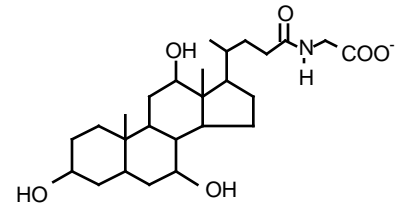
GLYCOCHOLATE
