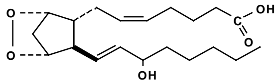
PGH 2
