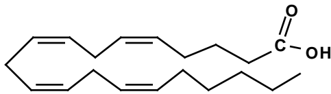
ARACHIDONIC ACID
