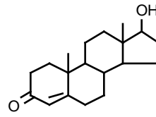
TESTOSTERONE
