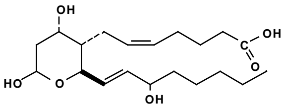
THROMBOXANE B 2
