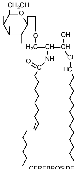
CEREBROSIDE
